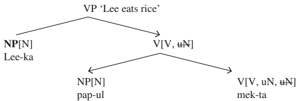
Figure 1.6. C-command
