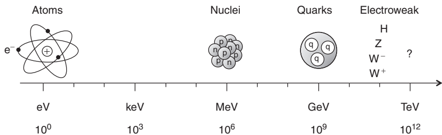
Fig. 1.1 The Universe at different energy scales, from atomic physics to modern particle physics at the TeV scale.
