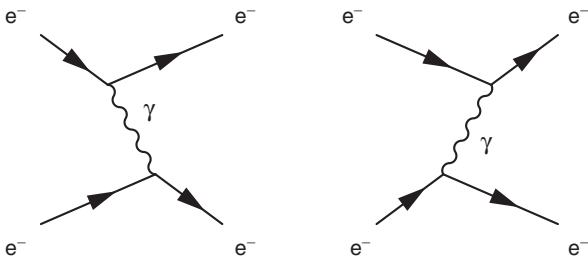
Fig. 1.3 The scattering of two electrons in QED by the exchange of a photon. With time running from left to right, the diagrams indicate the two possible time-orderings.
