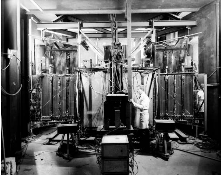
Figure 1.2 PS11, an optical spark chamber experiment at CERN's Proton Synchrotron, with accidental cosmic rays tracks. Picture CERN (1967).
