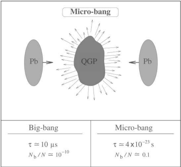
Fig. 1.1. Top: Lorentz-contracted nuclei collide in the center-of-momentum frame and form a region of dense matter, which evolves into a final state of hadrons. Bottom: two key differences involving baryon number N_b and total particle number N between the micro-bang and the cosmological big-bang.
