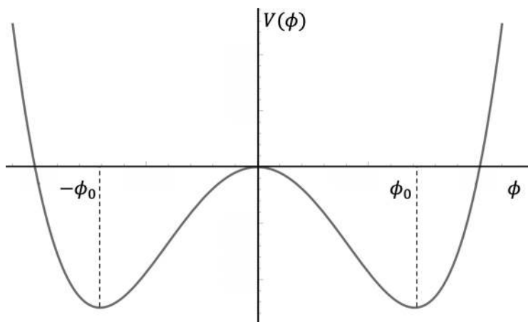
Figure 1.2 \mu^2\phi^2 - \lambda\phi^4 potential with \mu^2 < 0
