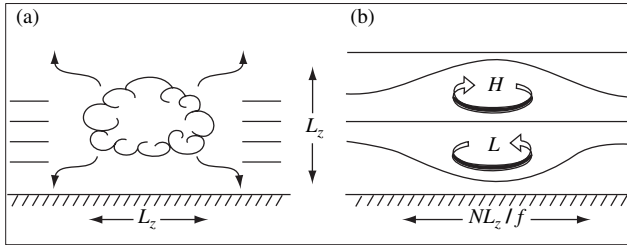
Fig. 1.5 Energy transfer process through geostrophic adjustment in the response of the free atmosphere to a cumulus cloud, which radiates gravity waves that lead to a lens of less stratified air whose width is the Rossby radius of deformation ( NL_z/f ). (a) The response of the free atmosphere to a cumulus cloud is the formation of gravity waves away from the cloud, which, in turn, lead to the formation of (b) a lens of less stratified air whose width is the Rossby radius of deformation. (Adapted after Emanuel and Raymond 1984.)
