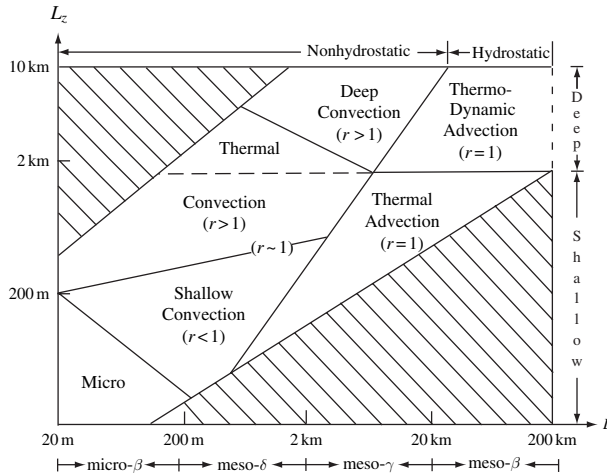
Fig. 1.2 Schematic of flow regimes under unstable stability conditions, where hatched zones indicate nonphysical flow regimes, the dotted line indicates merging of thermodynamic advection with macroscale, r represents scaled ratio of buoyancy and vertical pressure gradient forced perturbations, and the dashed line represents division of thermal convection into its deep and shallow regimes. (Adapted after Thunis and Bornstein 1996.)
