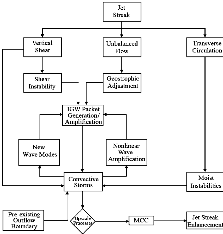
Fig. 1.4 Sketch of mutual interactions between the jet streak, inertial-gravity waves (IGW), and moist convection. (Adapted after Koch 1997.)
