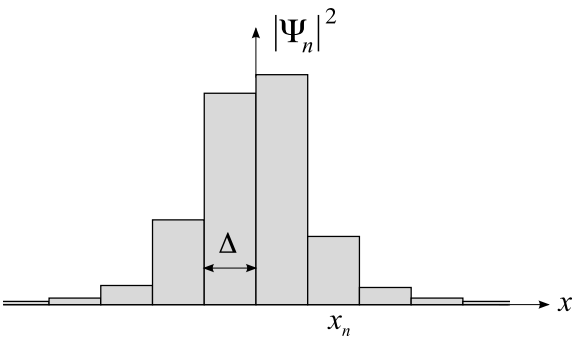
Figure 1.1 Histogram of the normalized number of clicks of the detector in x_n = n\Delta . The height of the function corresponds to the probability |\Psi_n|^2 .
