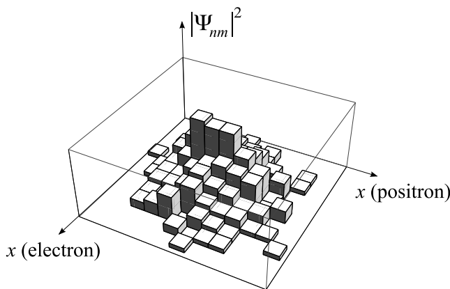
Figure 1.2 Histogram of the normalized number of simultaneous clicks of the electron and positron detectors in x_n = n\Delta and x_m = m\Delta respectively. The height of the function corresponds to the probability |\Psi_{nm}|^2 .
