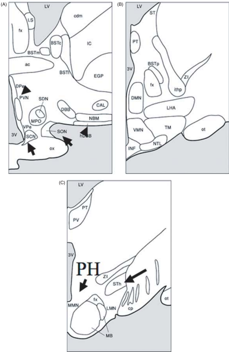
Figure 1.1 Scheme of the hypothalamic area. Arrows indicate the structures mentioned in the text. NBM, nucleus basalis of Meynert; PH, posterior hypothalamus; PVN, paraventricular nucleus; SCN, supraoptic nucleus; SON, supraoptic nucleus; STh, subthalamic nucleus.
