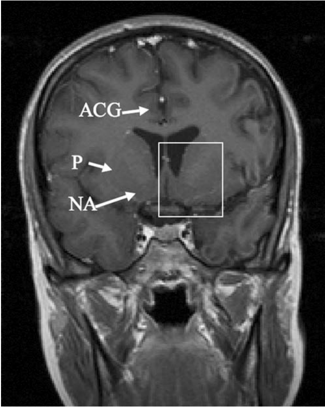
Figure 1.3 Frontal MRI scan. The white square indicates the hypothalamic area that is shown in more detail in Figure 1.1. ACG, anterior cingulate gyrus; NA, nucleus accumbens; P, putamen.
