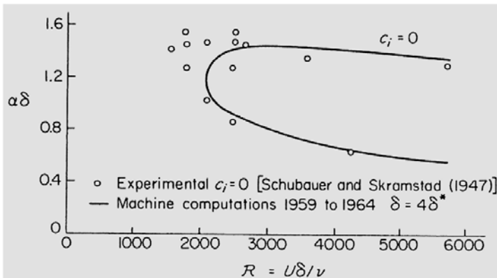
Fig. 1.4. Experimental and theoretical stability results for neutral oscillations of the Blasius boundary layer (after Betchov & Criminale, 1967).
