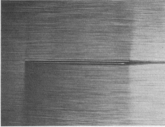
Fig. 1.1. Laminar Boundary Layer (after van Dyke, 1975).
