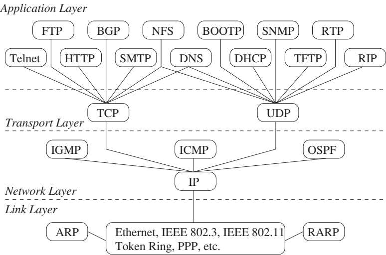
Figure 0.2. The TCP/IP protocols.
