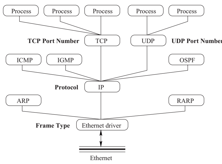
Figure 0.7. Multiplexing/demultiplexing in the layers.
