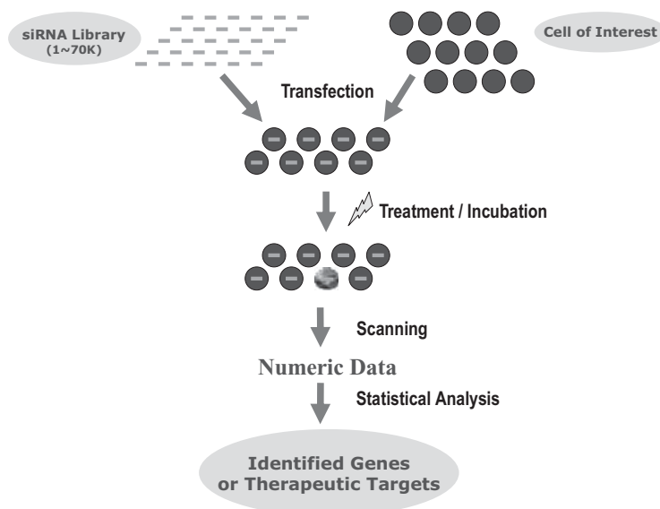
Figure 1.3 Procedure of genome-scale RNAi screens.
