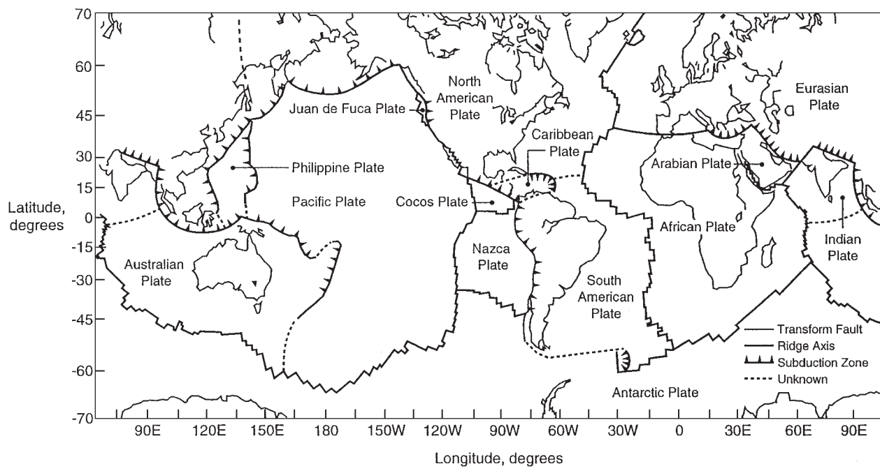
Figure 1.1 Distribution of the major plates. The ocean ridge axis (accretional plate margins), subduction zones (convergent plate margins), and transform faults that make up the plate boundaries are shown.
