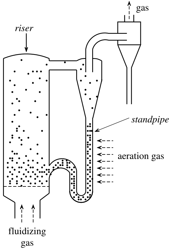
Fig. 1.1. This figure shows schematically one of several different configurations of a circulating fluidized bed loop used in engineering practice. The particles flow downward through the aerated “standpipe,” and enter the bottom of a fast fluidized bed “riser.” The particles are centrifugally separated from the gas in a train of “cyclones.” In this diagram, the particles separated in the primary cyclone are returned to the standpipe while the fate of the particles removed from the secondary cyclone is not shown.
