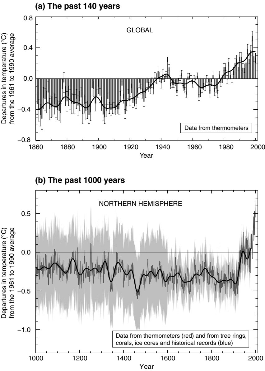
Figure 1.2. Variations of the surface temperature of the Earth over the last 140 years and the last millennium. The black line in (a) represents a decade by decade curve, in (b) the 50 years average variations. The thin whisker bars in (a) and the grey shaded area in (b) represent the 95% confidence range. For the difference between the direct data sources (thermometer, red) and indirect data sources (tree rings, corals, ice cores, historical records, blue), we refer to the original publication or website http://www.grida.no/climate/ipcc_tar/wg1/figspm-1.htm . Source: Houghton et al. (2001).
