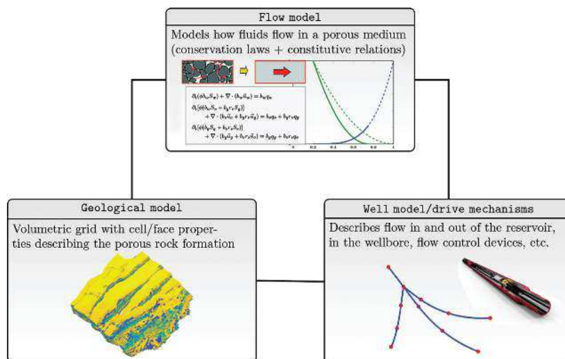
Figure 1.3 The three main constituents of a reservoir simulation model.
