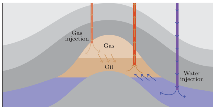
Figure 1.2 Conceptual illustration of voidage replacement, which is an example of a secondary production strategy in which gas and/or water is injected to maintain the reservoir pressure.
