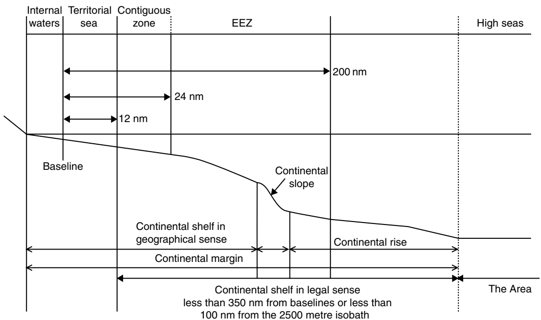
Figure 1.2. The case where the outer edge of the continental margin extends beyond 200 nautical miles from the baselines
