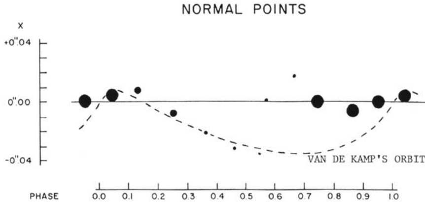
FIGURE 2. Refutation of a planetary companion to Barnard's Star, based on an independent data set and astrometric analysis (Gatewood & Eichhorn 1973). The size of the data points indicates their weight in the astrometric solution—smaller data points have larger errors. Only one astrometric axis ( x ) is shown.
