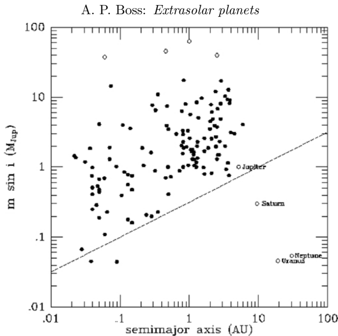
FIGURE 4. Extrasolar planet discovery space as of May 2005, showing primarily minimum masses of planets discovered by Doppler spectroscopy as a function of orbital semimajor axis. The oblique dashed line shows how the sensitivity limit of Doppler spectroscopy depends on semimajor axis for accuracies of \sim 2\text{--}3 \text{ m s}^{-1} and a signal-to-noise ratio of \sim 4 —short-period, massive planets are the easiest to detect. Brown dwarfs (open symbols near the top of discovery space) are infrequent companions to solar-type stars.
