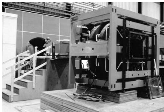
Figure 1.4 0.15T resistive magnet used by Philips in the early development of MRI. Courtesy of Philips Medical Systems.
