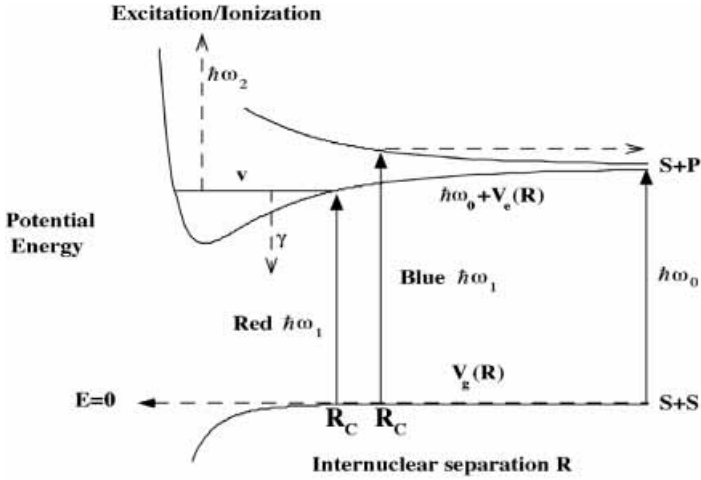
Fig. 1.2. Schematic of a cold collision. Light field \hbar\omega_1 , red detuned with respect to the S + P asymptote, excites the quasimolecule in a free-bound transition around the Condon point R_C and can lead to excitation or ionization with the absorption of a second photon \hbar\omega_2 . Light field \hbar\omega_1 , blue detuned with respect to the S + P asymptote, prevents atoms from approaching significantly beyond the Condon point. Blue-detuned excitation leads to optical shielding and suppression of inelastic and reactive collision rates.
