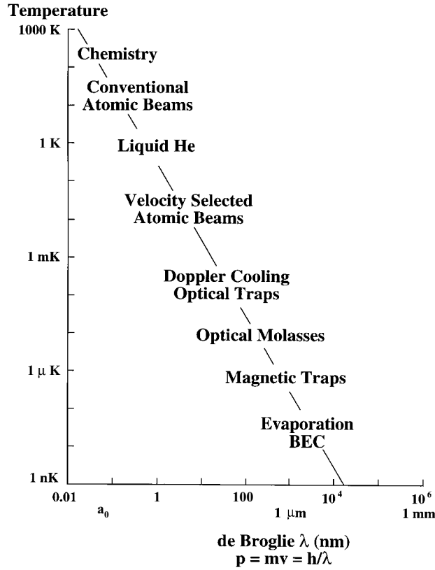
Fig. 1.1. Illustrative plot of various physical phenomena along a scale of temperature (energy divided by Boltzmann's constant k_B ) plotted against the de Broglie wavelength for atomic sodium.
