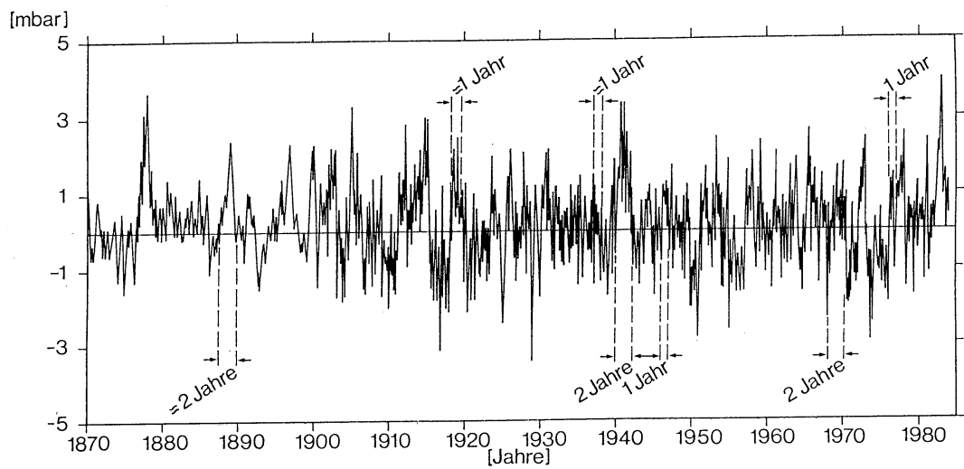
Figure 1.2: The monthly mean Southern Oscillation Index, computed as the difference between Darwin (Australia) and Papeete (Tahiti) monthly mean sea-level pressure ('Jahr' is German for 'year').
