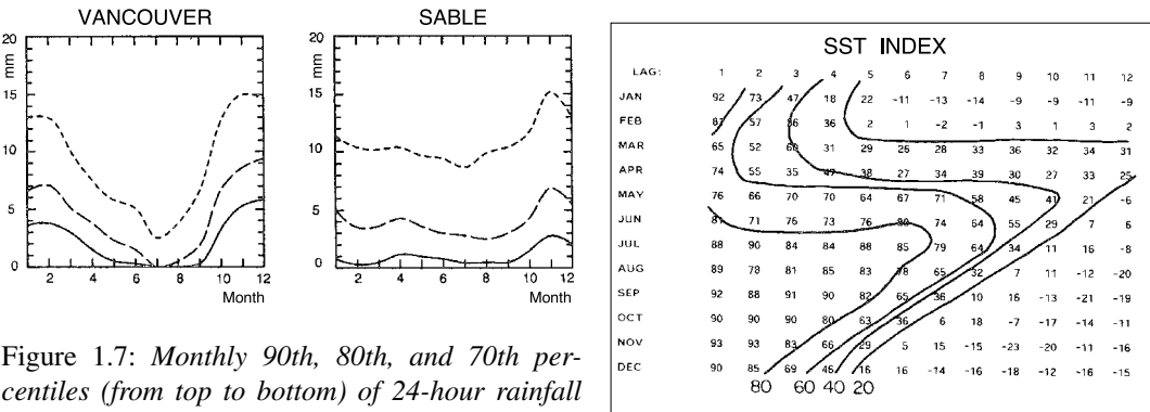
Figure 1.8: Seasonal dependence of the lag correlations of the SST index of the Southern Oscillation. The correlations are given in hundreds so that isolines represent lag correlations of 0.8, 0.6, 0.4, and 0.2. The row labelled 'Jan' lists correlations between January values of the index and the index observed later 'lag' months [427].
