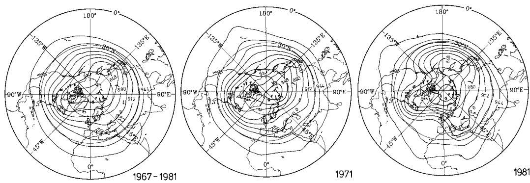
Figure 1.1: The 300 hPa geopotential height fields in the Northern Hemisphere: the mean 1967–81 January field, the January 1971 field, which is closer to the mean field than most others, and the January 1981 field, which deviates significantly from the mean field. Units: 10 m [117].
