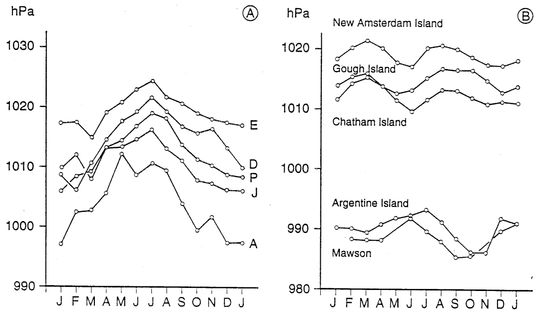
Figure 1.6: Annual cycle of sea-level pressure at extratropical locations. a) Northern Hemisphere Ocean Weather Stations: A = 62° N, 33° W; D = 44° N, 41° W; E = 35° N, 48° W; J = 52° N, 25° W; P = 50° N, 145° W. b) Southern Hemisphere.
