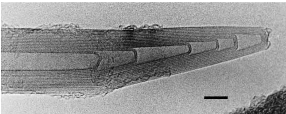
Fig. 1.5. Image of typical multiwalled nanotube cap. Scale bar 5 nm.
